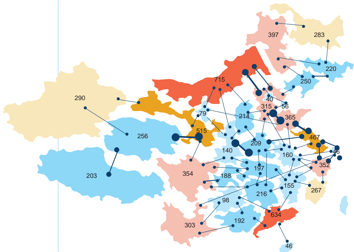
Figure 7 Inter-provincial Transmission Capacity Demand and the Total Installed Capacity of Each Province (GW) in High Penetration Scenario
