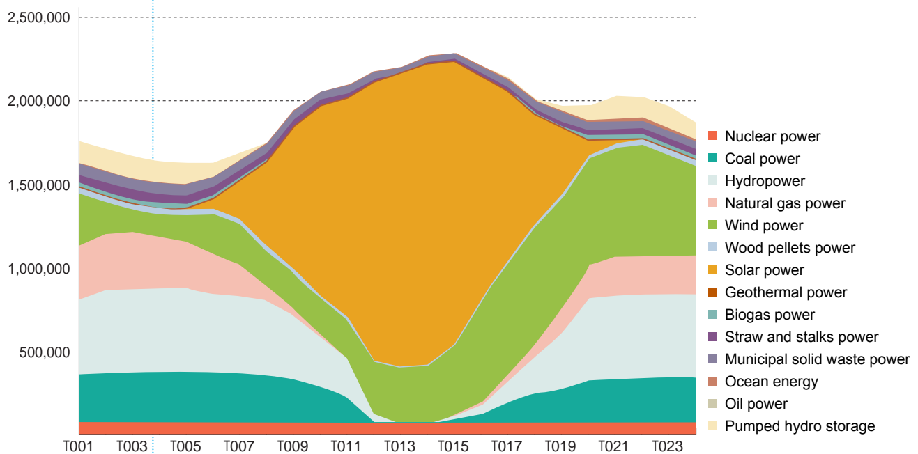
Figure 8 Analysis of the Hourly Dispatch of Nationwide Power Generation on a Typical Day in High Penetration Scenario
