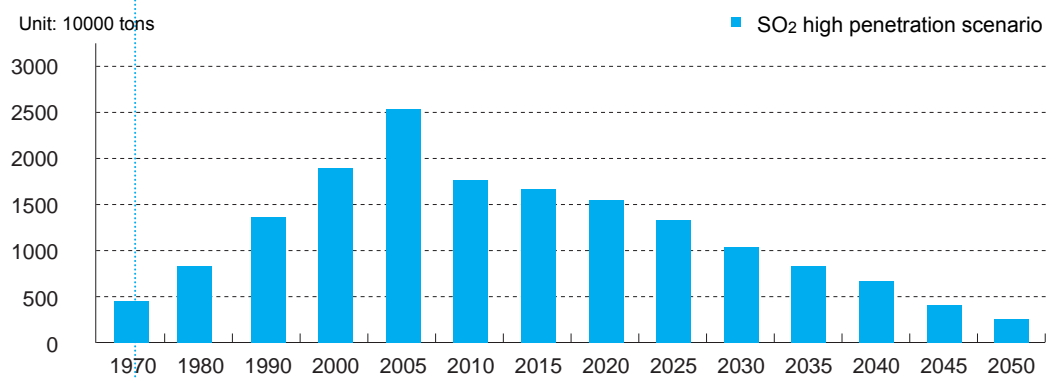
Figure 11-3 China's SO 2 Emission in High Penetration Scenario
