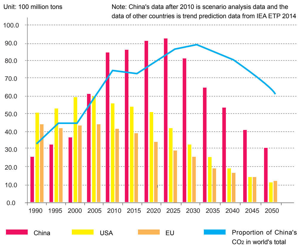
Figure 11-1 China's CO 2 Emission in the Global Contrast in High Penetration Scenario
