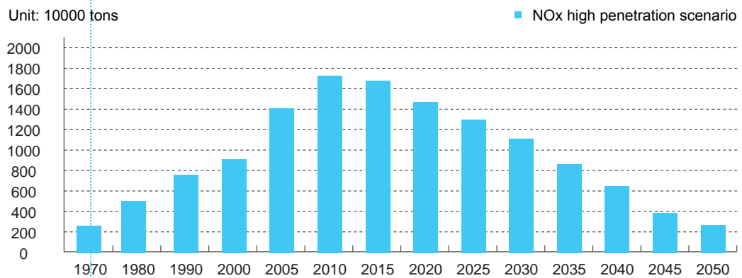
Figure 11-2 China's NOx Emission in High Penetration Scenario
