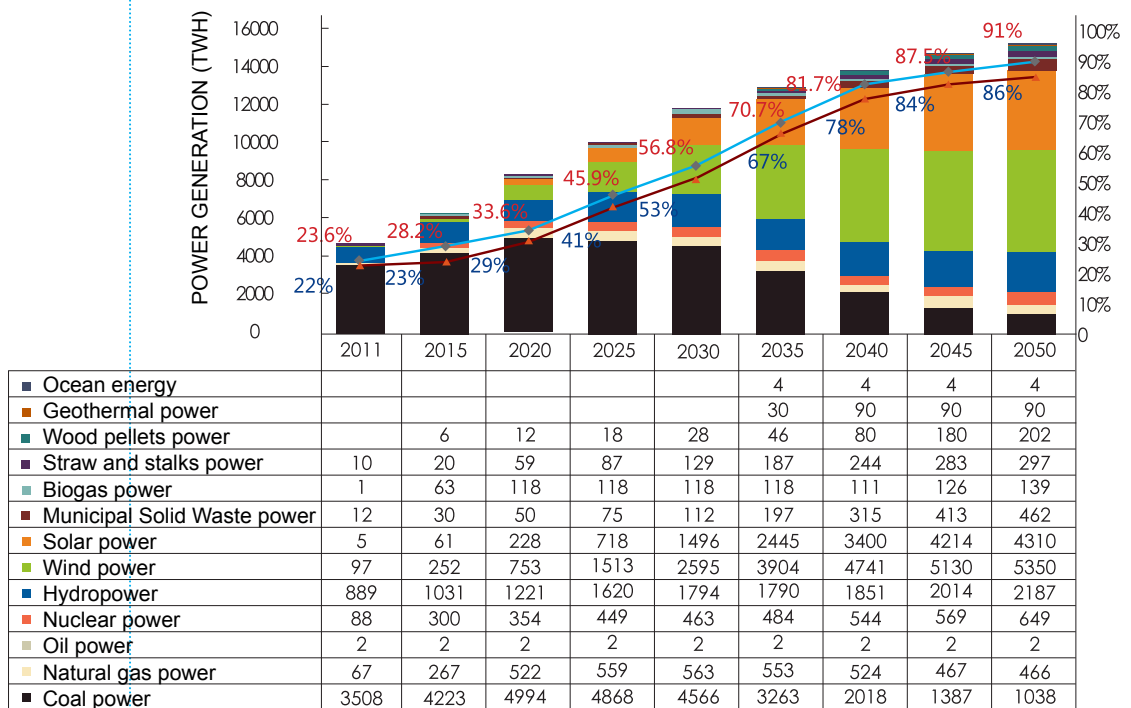
Figure 4 Power Generation in High Penetration Scenario
