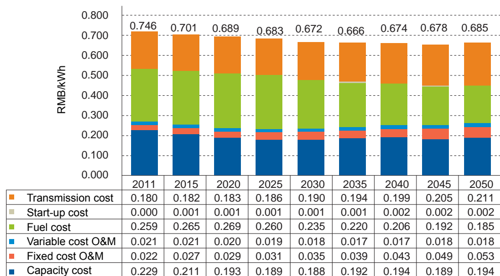
Figure 9 Trend of kWh Cost Development in High Penetration Scenario
