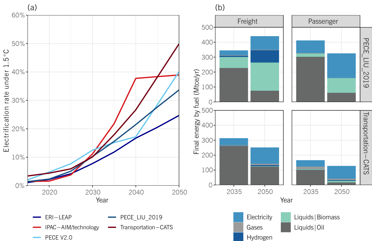
FIGURE 4-19. ELECTRICITY PERCENTAGE IN TOTAL TRANSPORTATION ENERGY CONSUMPTION (PANEL A) AND TWO ILLUSTRATIVE SCENARIOS OF ENERGY DEMAND AND FUEL MIX IN THE TRANSPORTATION SECTOR (PANEL B).
